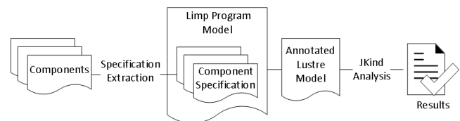
Figure 1: SIMPAL architecture flow.
