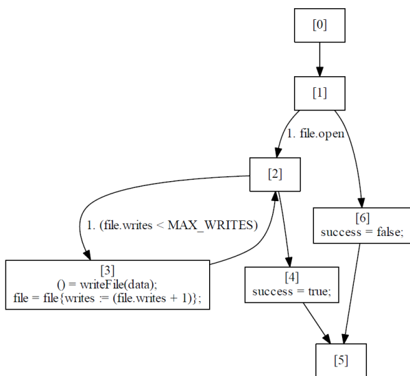
Figure 3: Control flow graph for Figure 2
